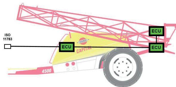
ISO compatible sprayer layout showing three Electronic Control Units.
