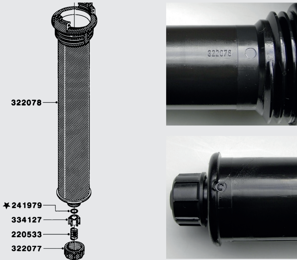
Synthetic cylinder for hand-operated pump: C indicates the 4th version
