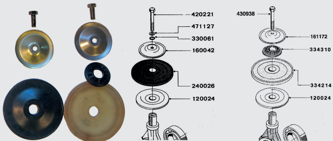
Older (black) and new version (yellow) diaphragm for model 1200 and 1300 series pumps
