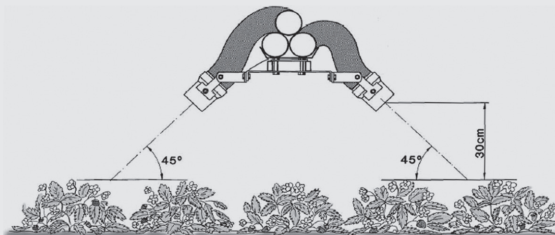
Setup guide from the instruction book of the 1982 MINI Variant with 10 spouts
