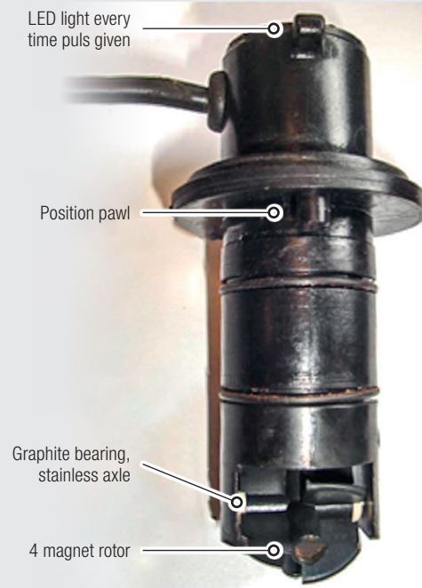
Flow sensor with rotor at bottom
